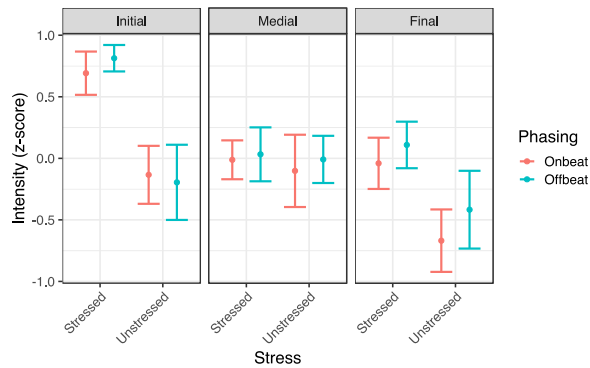
Figure 14: Vowel intensity as a function of phasing, word position, and stress; English speakers
