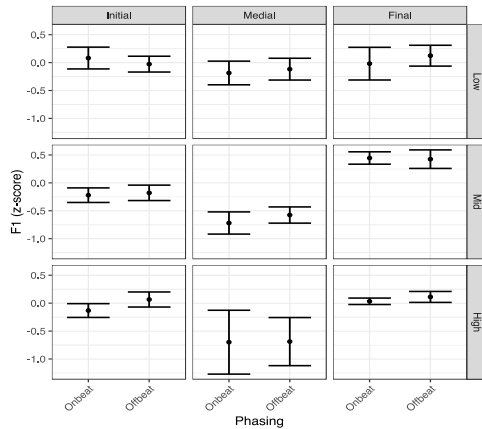
Figure 9: Vowel F1 as a function of phasing, word position, and tone; Medumba speakers
