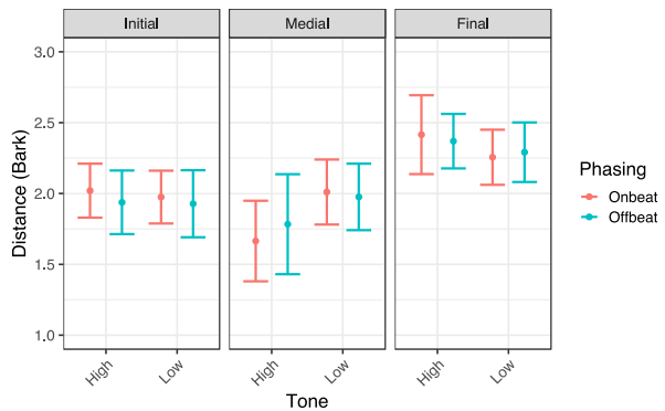
Figure 13: Euclidean distance as a function of phasing, word position, and tone; Medumba speakers
