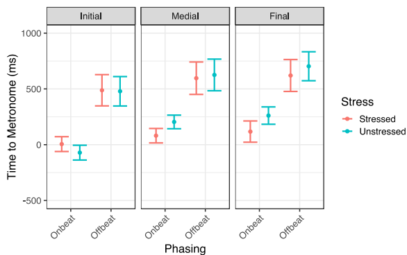
Figure 2: Metronome Distance as a function of phasing, word position, and stress; English speakers
