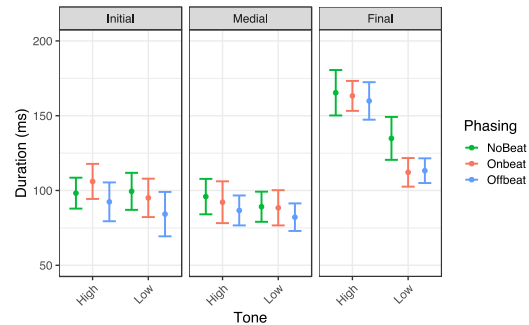
Figure 19: Vowel duration as a function of word phasing (3-way), word position, and tone, Medumba speakers
