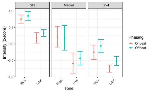
Figure 15: Vowel intensity as a function of phasing, word position, and stress; Medumba speakers
