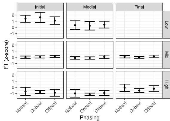
Figure 21: F1 as a function of phasing (3-way), position, and vowel height, English speakers
