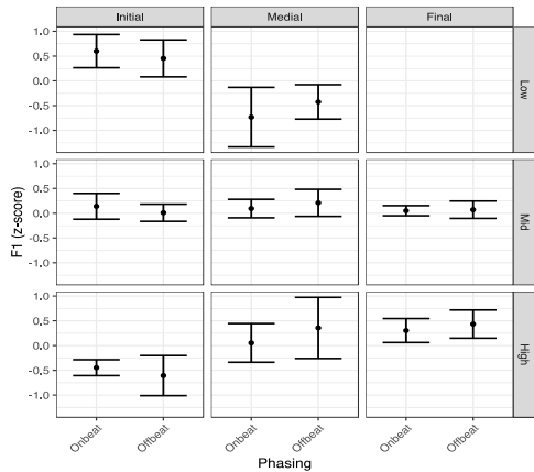
Figure 8: Vowel F1 as a function of phasing, word position, and stress; English speakers
