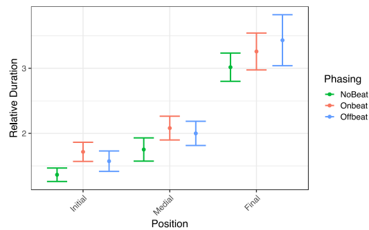
Figure 20: Relative duration (ratio of stressed to unstressed vowel duration) across positions and phasing conditions
